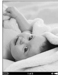
Picture viewer
